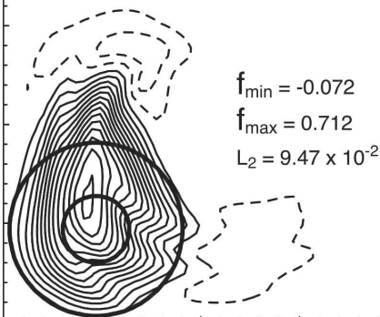
(a) Time-split PPM, 50 x 50 Cr_{\max} = 1
