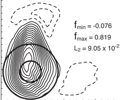
(b) Strang-split PPM, 50 x 50 Cr_{\max} = 1
